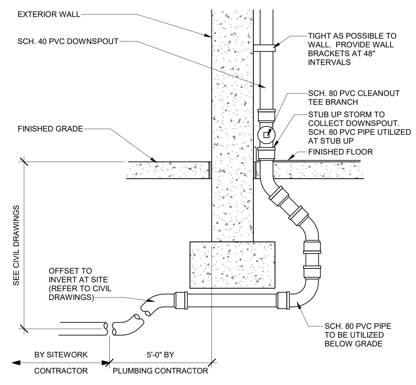
9 building downspout (interior) SCALE | N.T.S.
