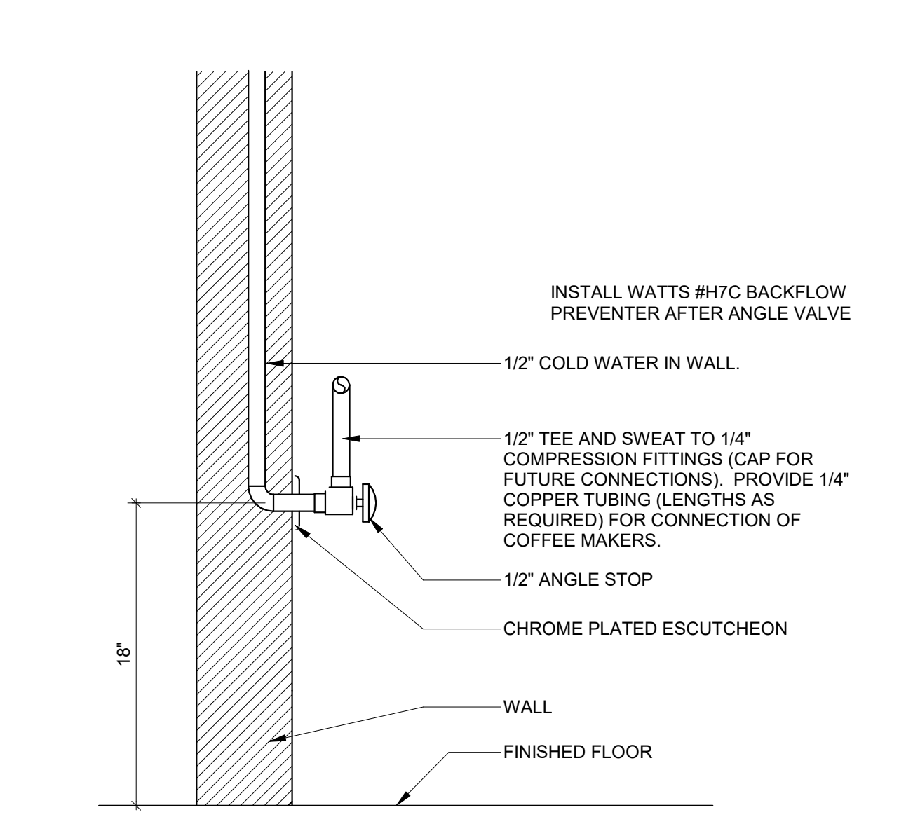
4 coffee maker supply SCALE | N.T.S.
