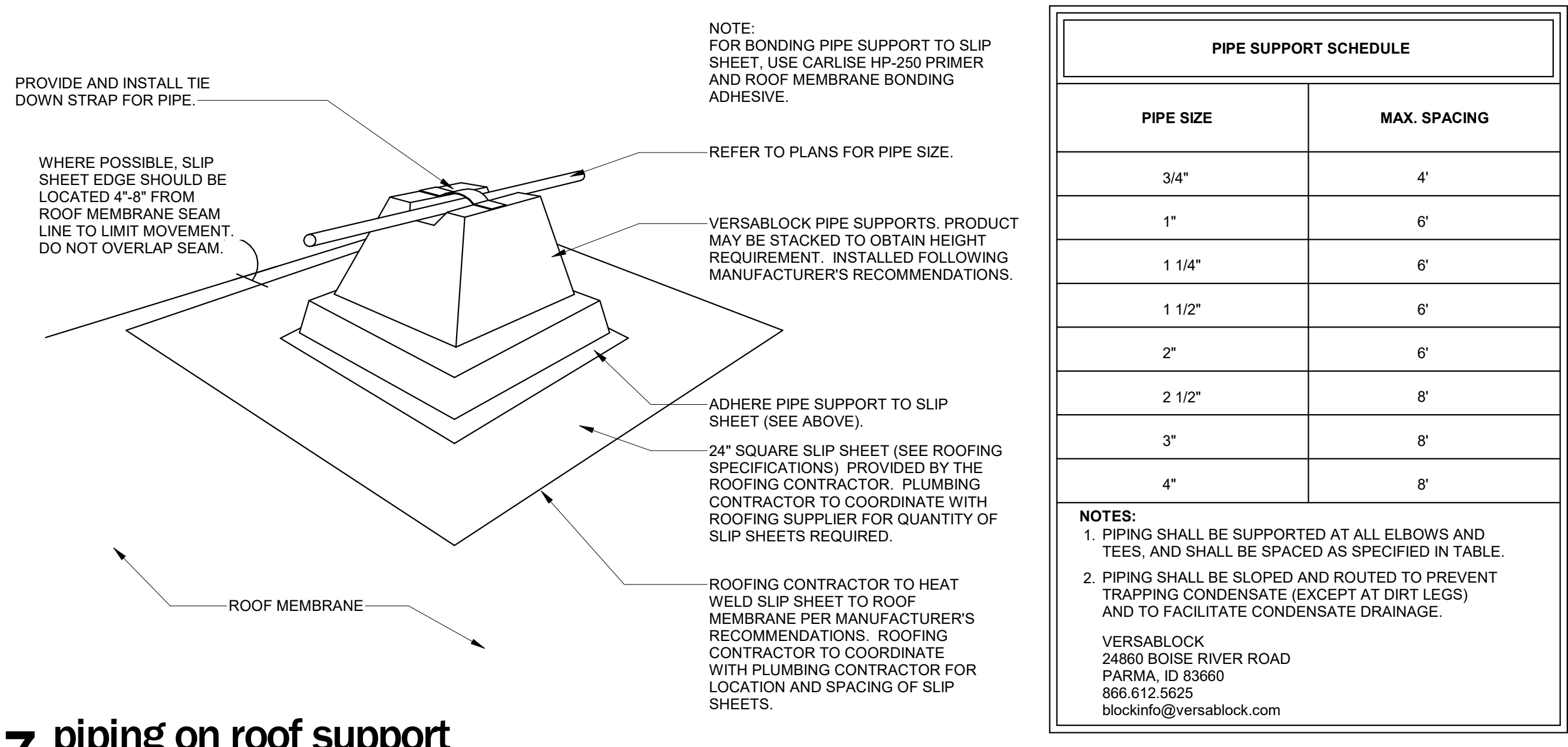
7 piping on roof support SCALE | N.T.S.
