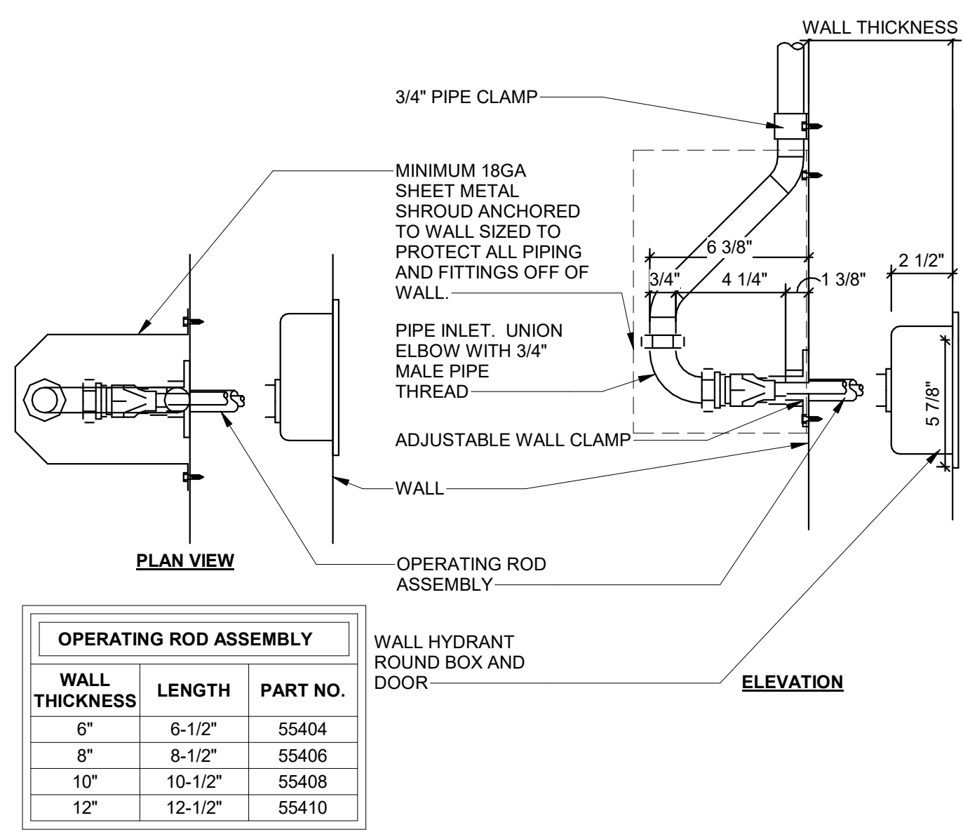
1 wall hydrant (WH-1) SCALE | N.T.S.
